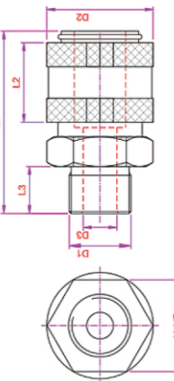
COUPLER ( BSP(M) )
