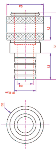
COUPLER ( HOSE )
