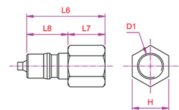
ADAPTOR ( BSP(F) )
